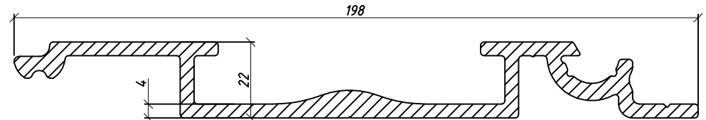
Alu 8/160 Leak Proof T subdeck (Turn-in)
